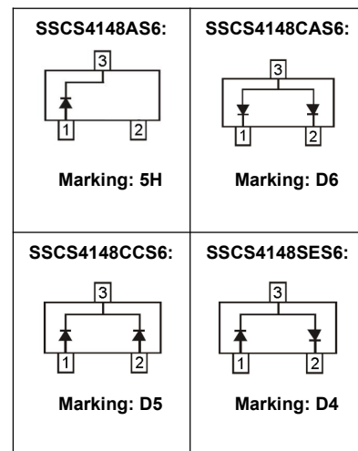
Circuit Diagram
